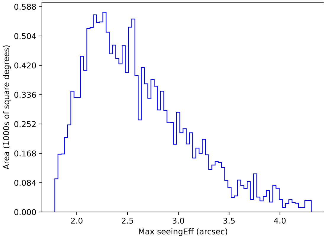
internal_u_expt30_nscale1.2v3.4_10yrs WFD u band: Max seeingEff
