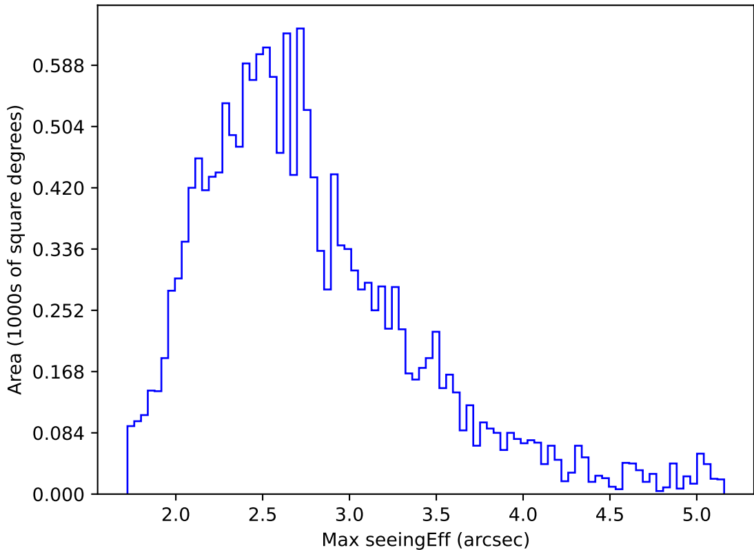
internal_u_expt30_nscale1.2v3.4_10yrs WFD i band: Max seeingEff
