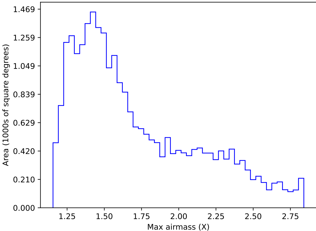
internal_u_expt30_nscale1.2v3.4_10yrs Yr 1 z band: Max airmass
