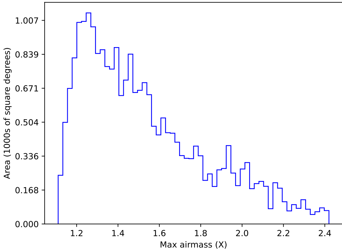
internal_u_expt30_nscale1.2v3.4_10yrs Yr 1 u band: Max airmass
