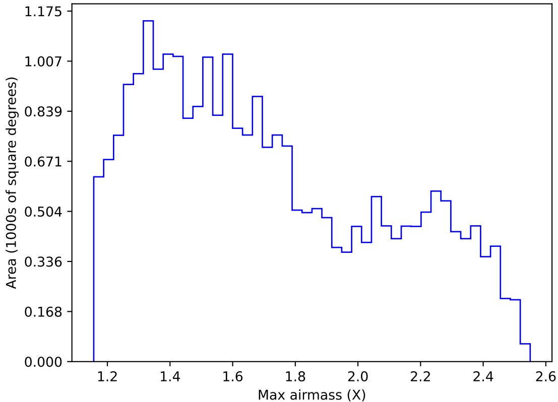
internal_u_expt30_nscale1.2v3.4_10yrs Yr 1 r band: Max airmass
