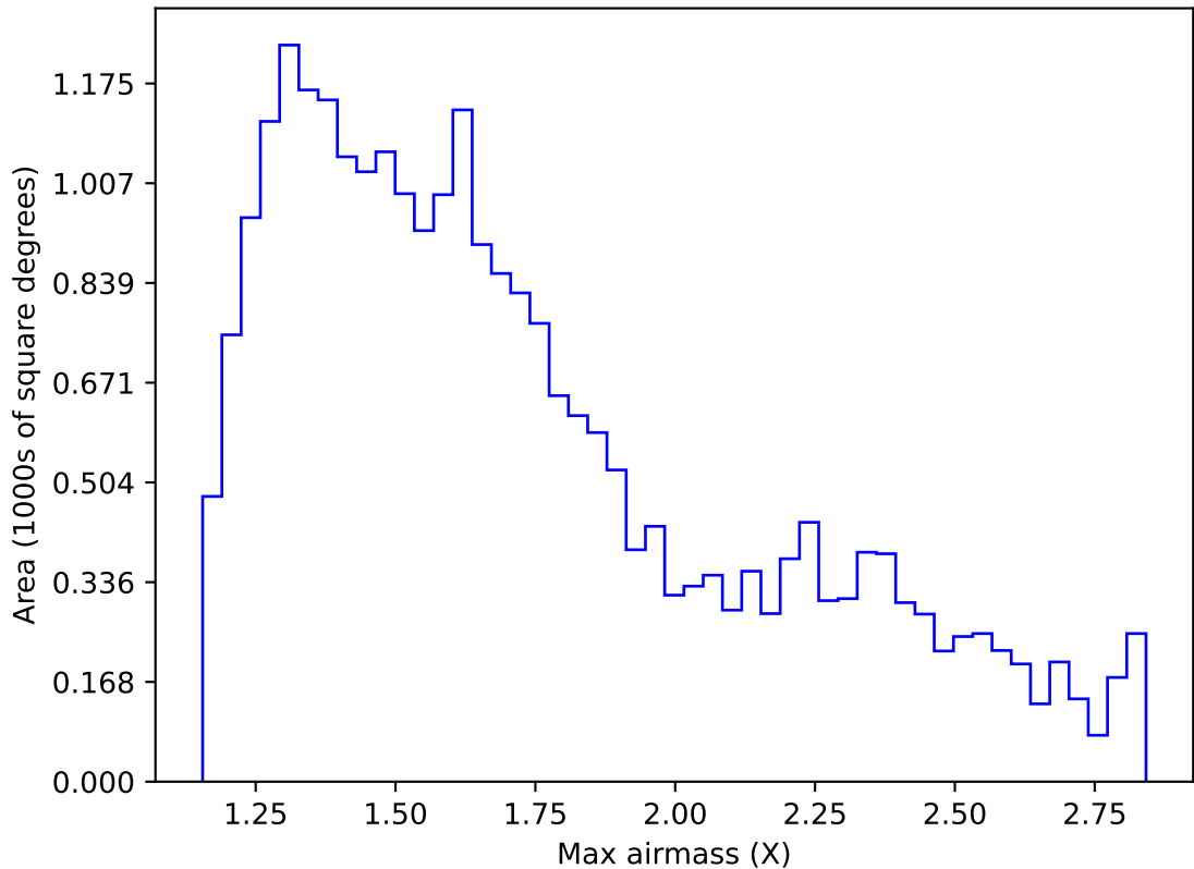
internal_u_expt30_nscale1.2v3.4_10yrs Yr 1 i band: Max airmass
