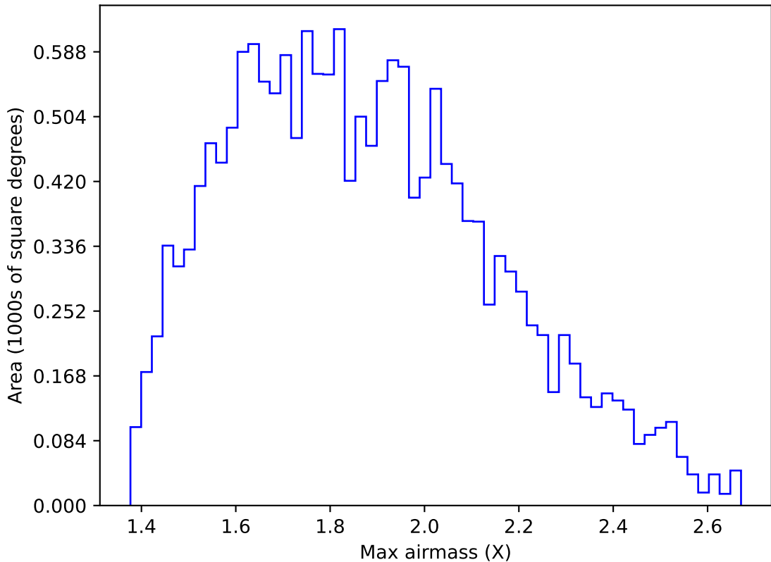
internal_u_expt30_nscale1.2v3.4_10yrs WFD u band: Max airmass
