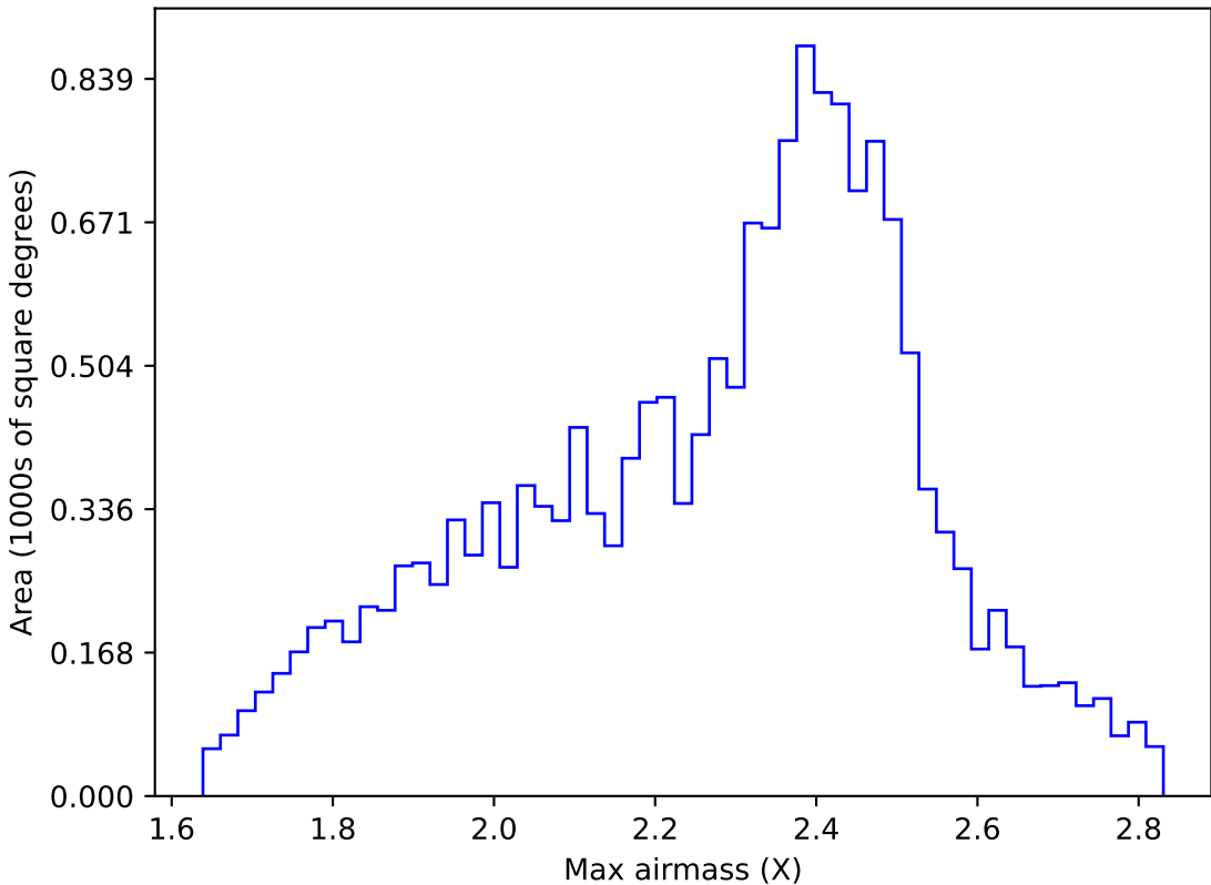
internal_u_expt30_nscale1.2v3.4_10yrs WFD r band: Max airmass
