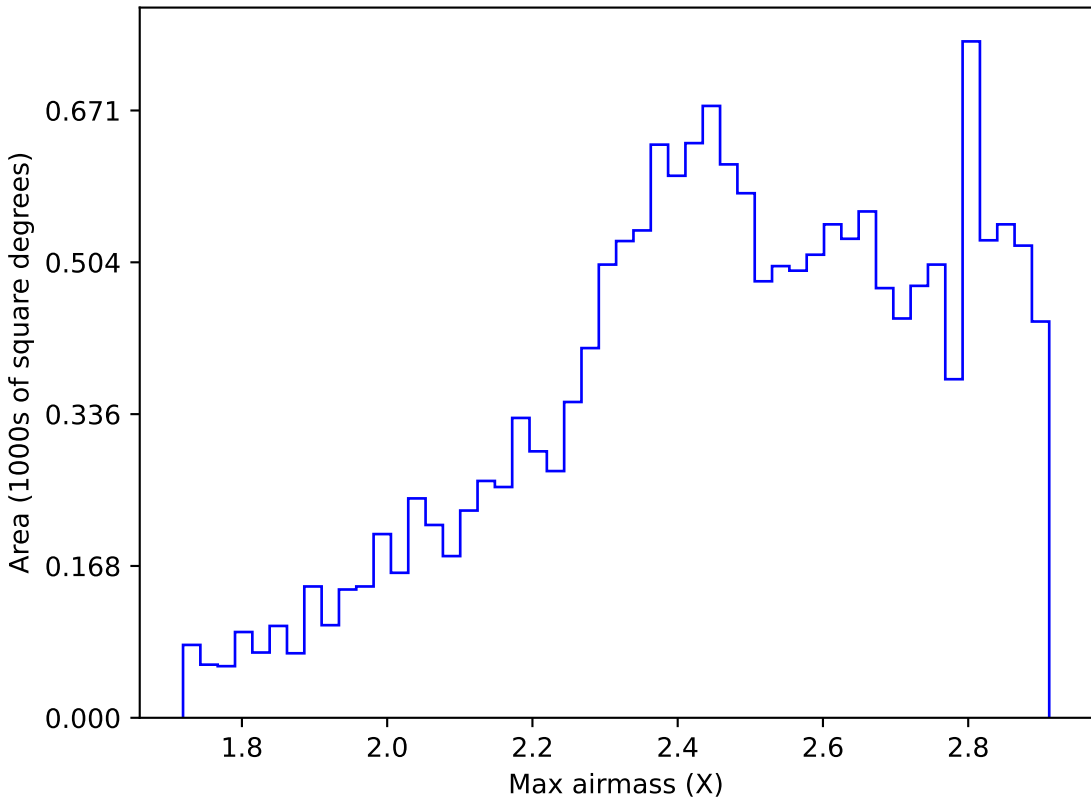
internal_u_expt30_nscale1.2v3.4_10yrs WFD i band: Max airmass
