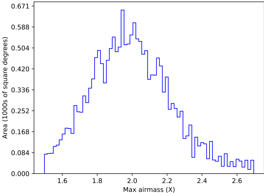
internal_u_expt30_nscale1.2v3.4_10yrs WFD g band: Max airmass
