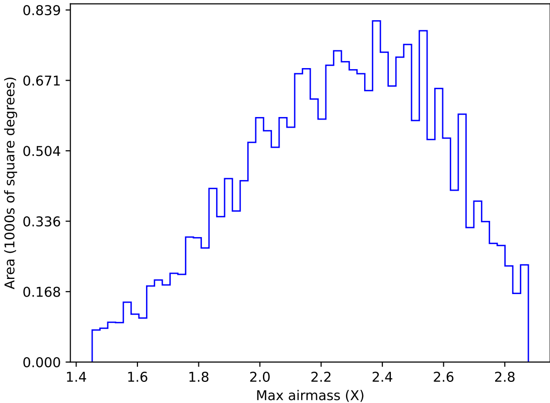
internal_u_expt30_nscale1.2v3.4_10yrs All sky y band: Max airmass
