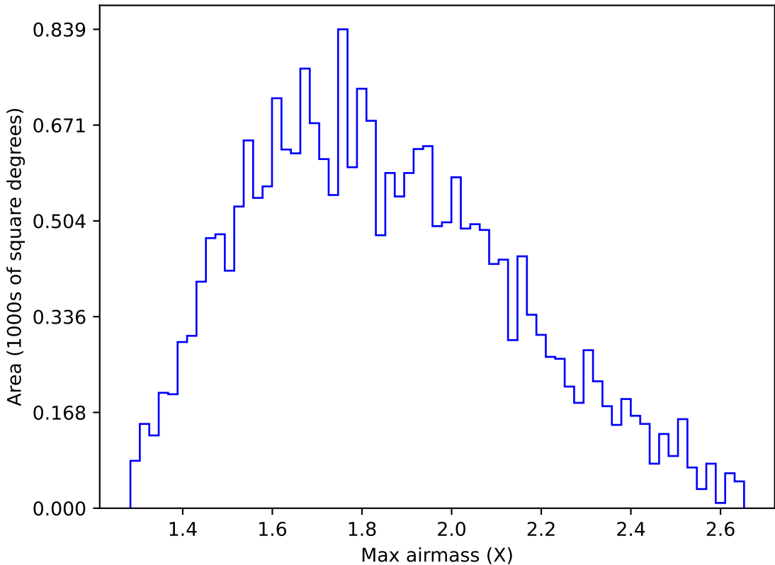
internal_u_expt30_nscale1.2v3.4_10yrs All sky u band: Max airmass
