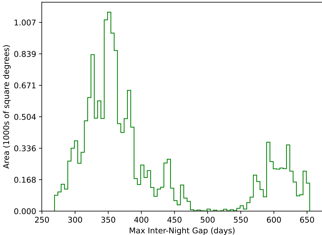
internal_u_expt30_nscale1.2v3.4_10yrs WFD g band: Max Inter-Night Gap
