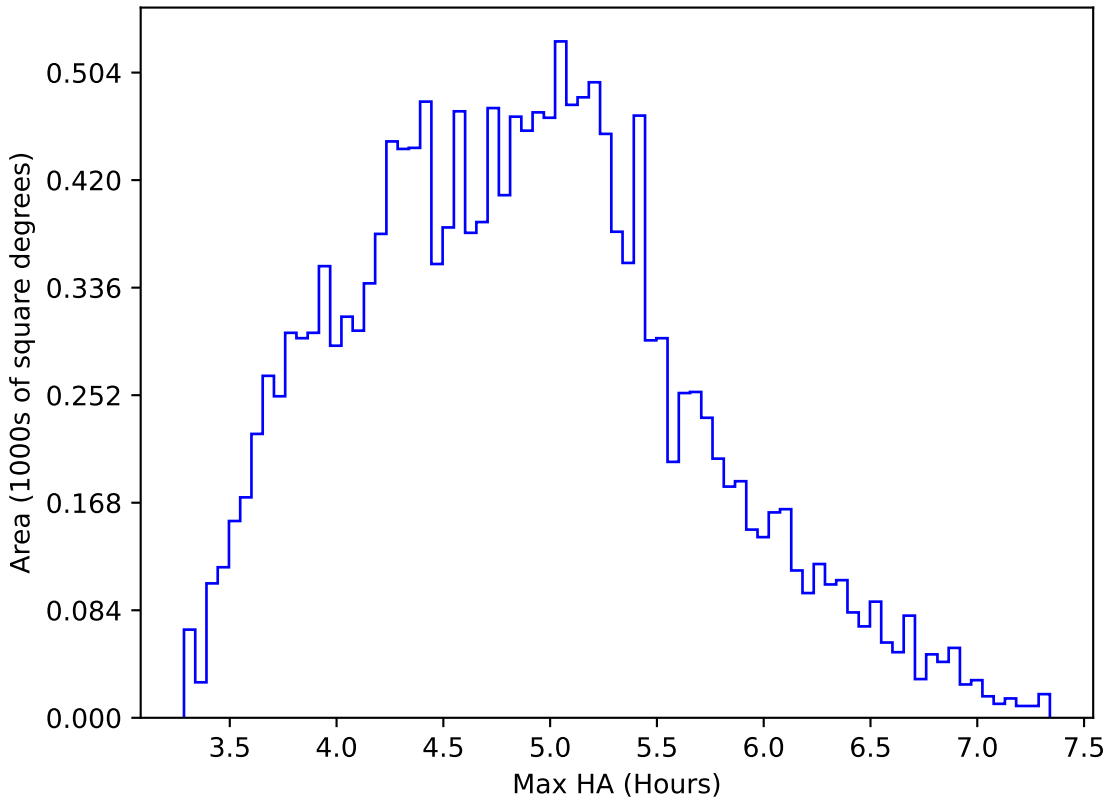
internal_u_expt30_nscale1.2v3.4_10yrs WFD z band: Max HA
