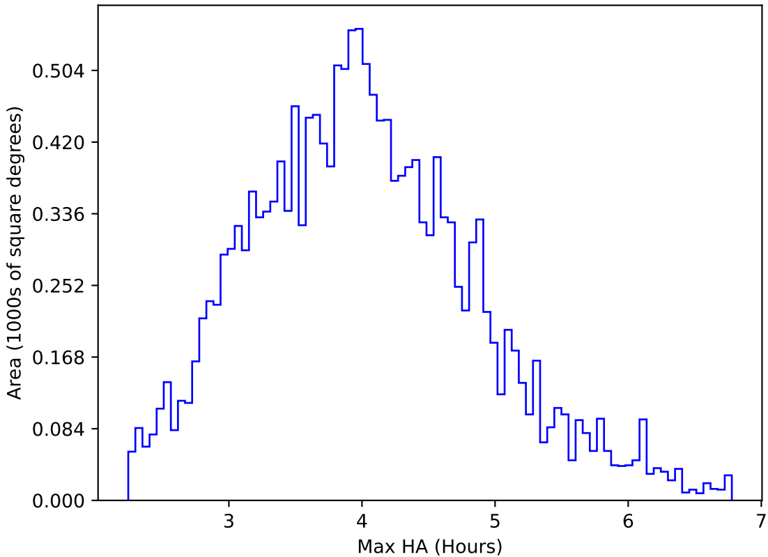
internal_u_expt30_nscale1.2v3.4_10yrs WFD u band: Max HA
