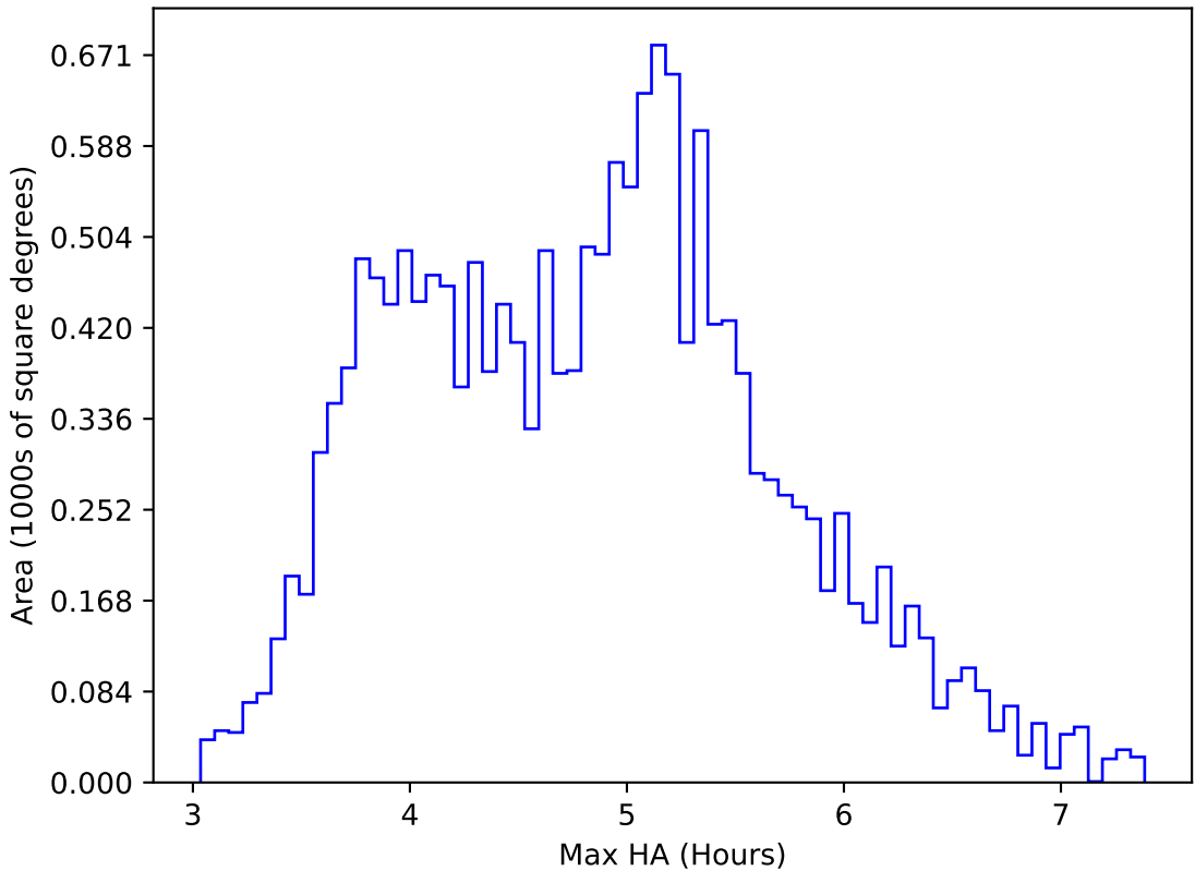
internal_u_expt30_nscale1.2v3.4_10yrs WFD i band: Max HA
