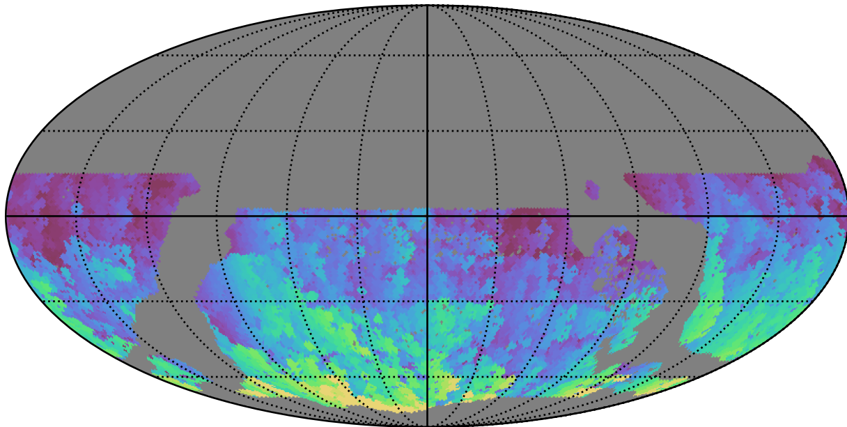
internal_u_expt30_nscale1.2v3.4_10yrs WFD g band: Max HA
