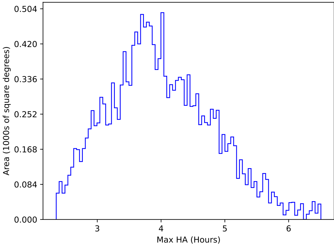
internal_u_expt30_nscale1.2v3.4_10yrs WFD g band: Max HA
