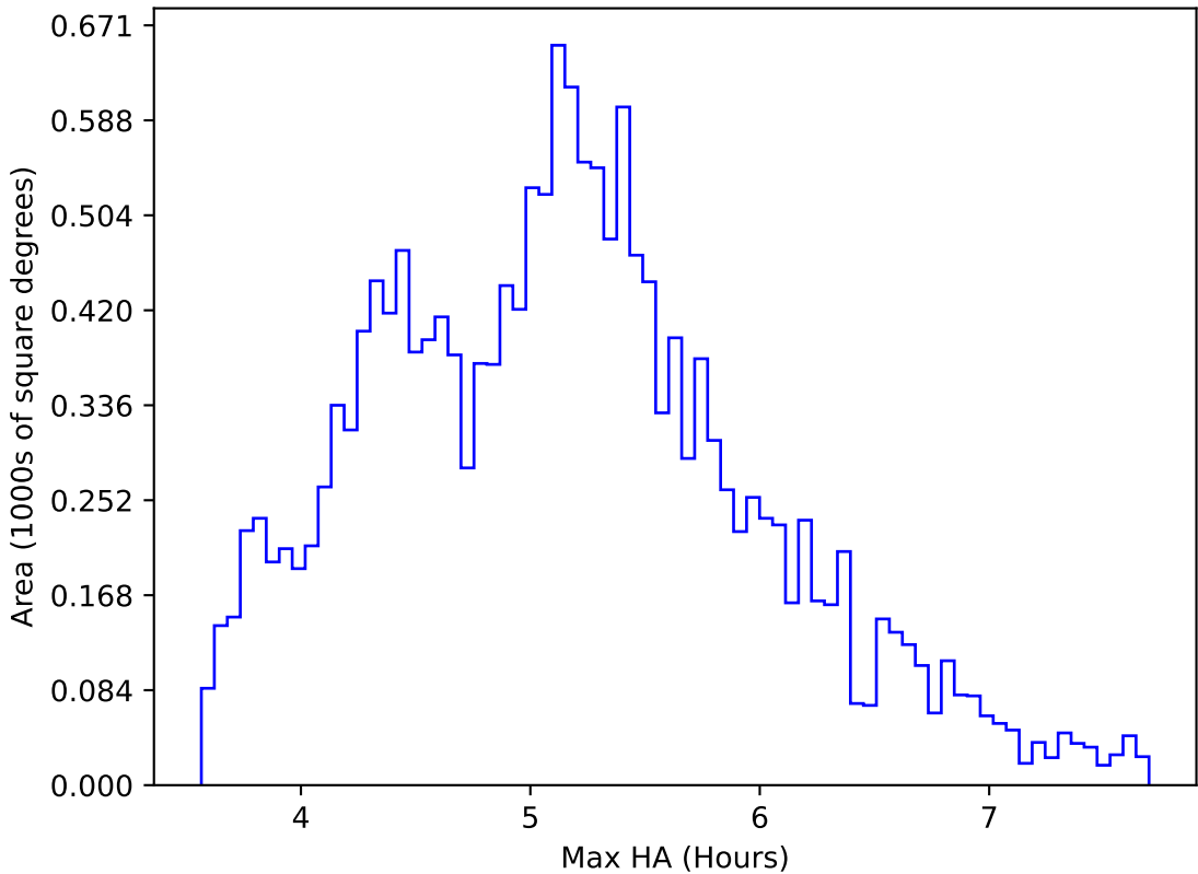
internal_u_expt30_nscale1.2v3.4_10yrs WFD all bands: Max HA
