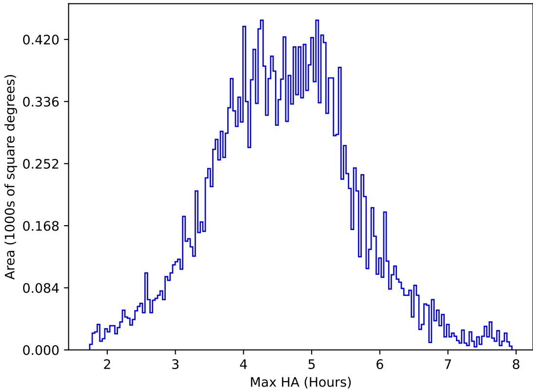
internal_u_expt30_nscale1.2v3.4_10yrs All sky z band: Max HA
