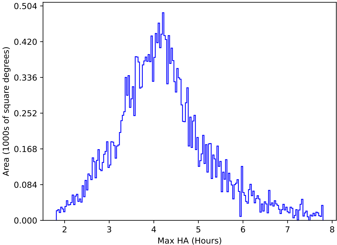
internal_u_expt30_nscale1.2v3.4_10yrs All sky r band: Max HA
