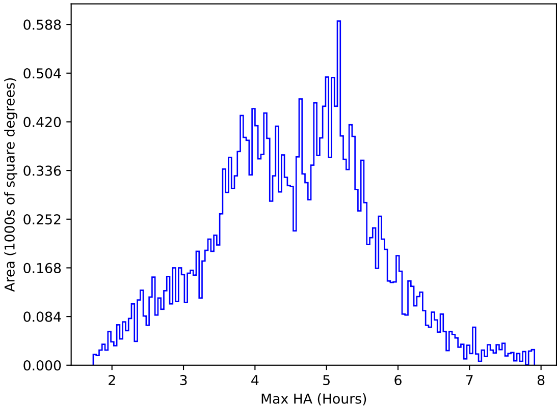
internal_u_expt30_nscale1.2v3.4_10yrs All sky i band: Max HA
