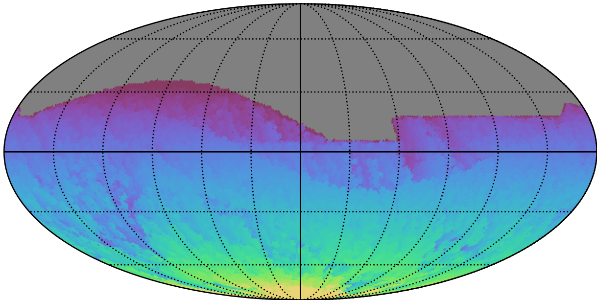
internal_u_expt30_nscale1.2v3.4_10yrs All sky all bands: Max HA
