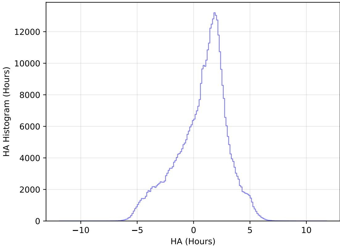
internal_u_expt30_nscale1.2v3.4_10yrs WFD z band: HA Histogram
