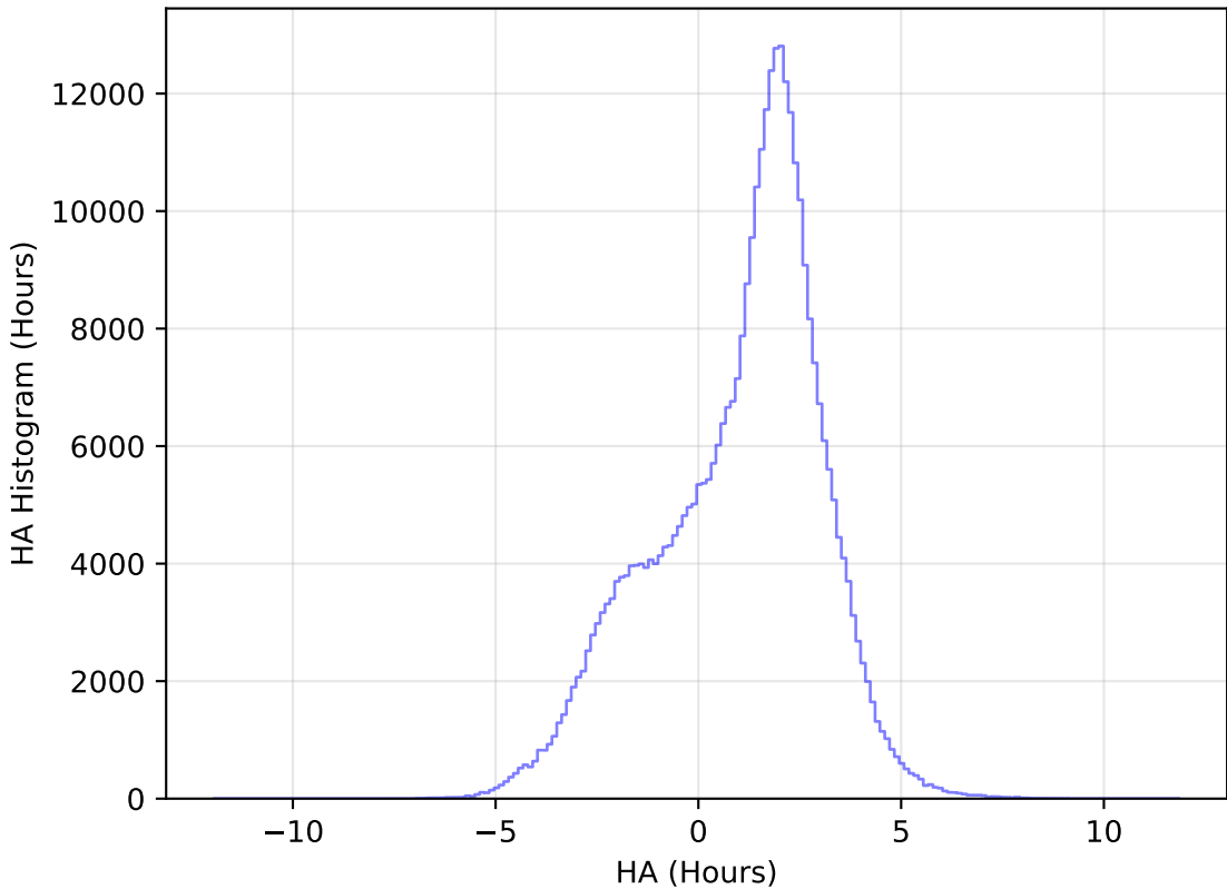
internal_u_expt30_nscale1.2v3.4_10yrs WFD y band: HA Histogram
