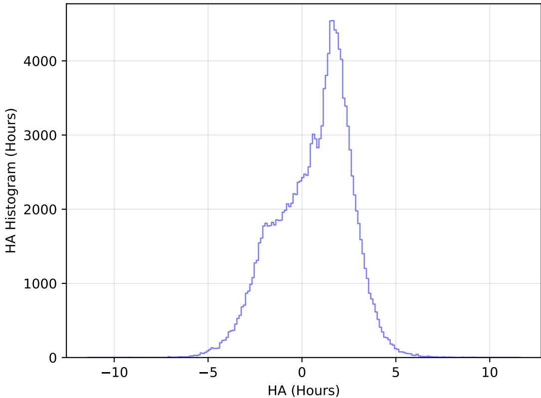
internal_u_expt30_nscale1.2v3.4_10yrs WFD u band: HA Histogram
