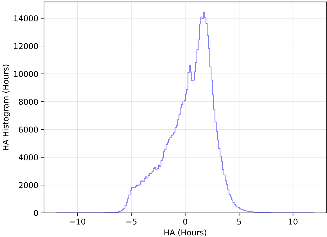
internal_u_expt30_nscale1.2v3.4_10yrs WFD r band: HA Histogram
