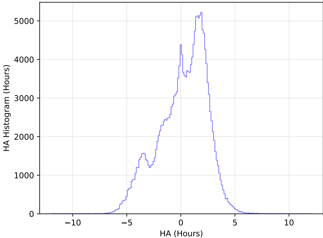
internal_u_expt30_nscale1.2v3.4_10yrs WFD g band: HA Histogram
