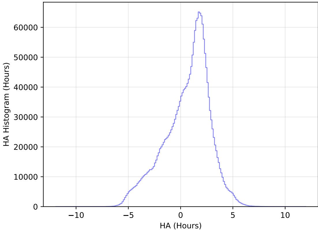
internal_u_expt30_nscale1.2v3.4_10yrs WFD all bands: HA Histogram
