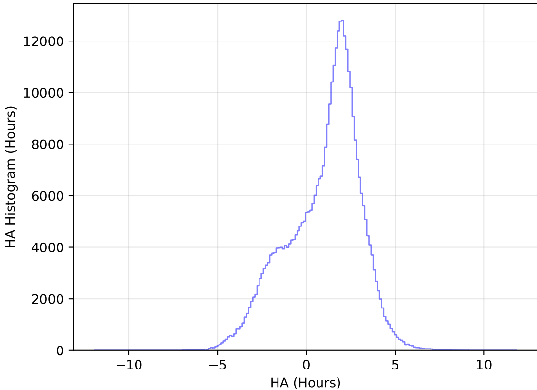
internal_u_expt30_nscale1.2v3.4_10yrs All sky y band: HA Histogram
