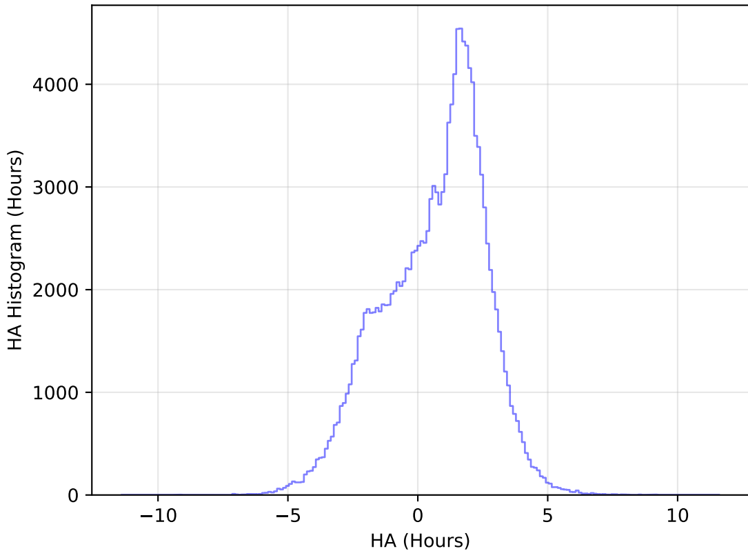
internal_u_expt30_nscale1.2v3.4_10yrs All sky u band: HA Histogram
