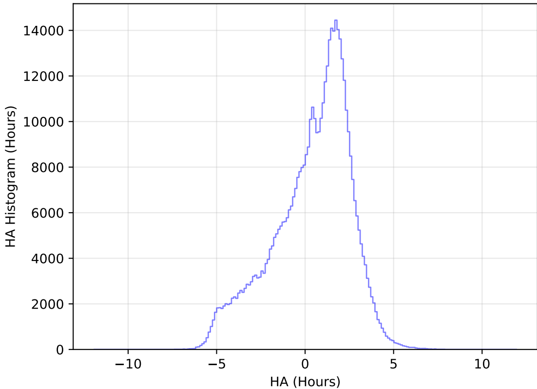
internal_u_expt30_nscale1.2v3.4_10yrs All sky r band: HA Histogram
