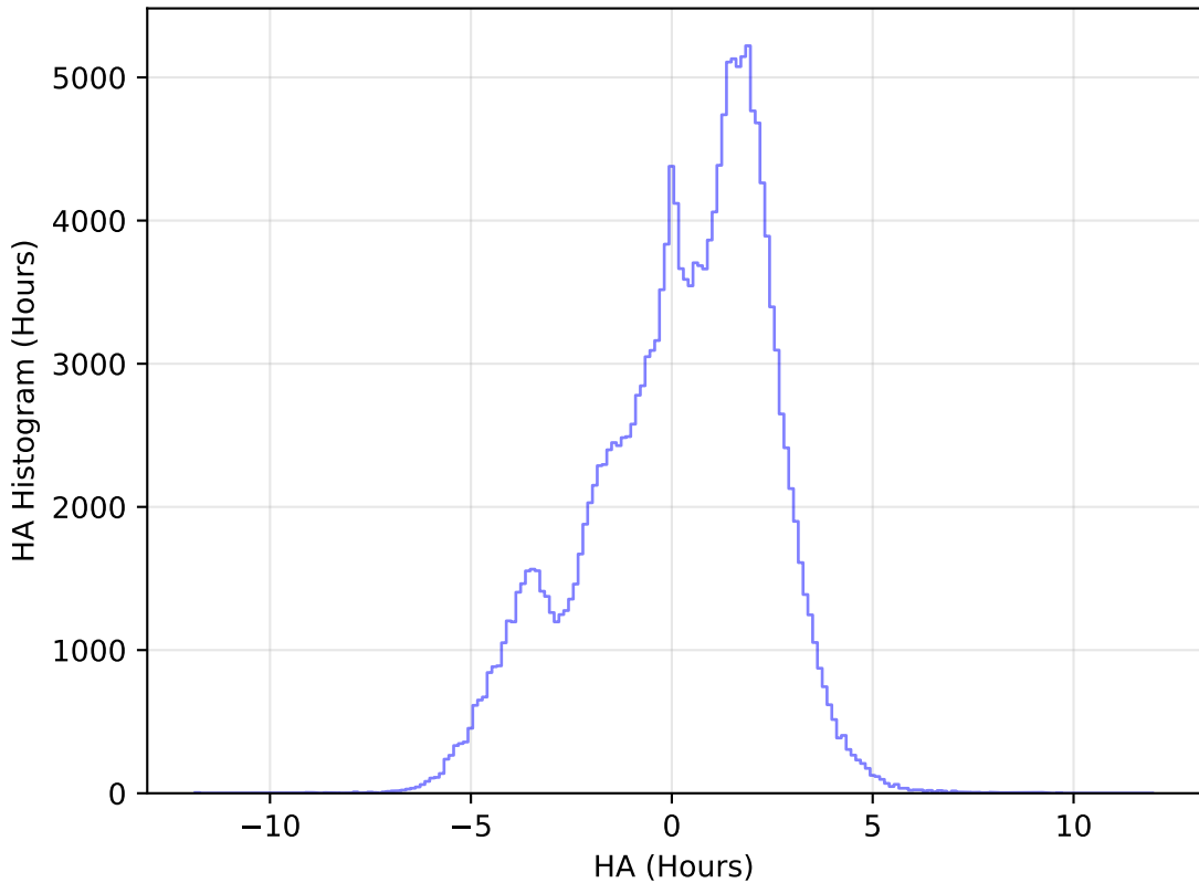
internal_u_expt30_nscale1.2v3.4_10yrs All sky g band: HA Histogram
