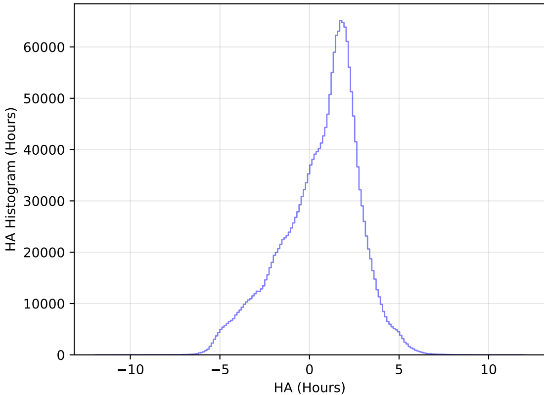
internal_u_expt30_nscale1.2v3.4_10yrs All sky all bands: HA Histogram
