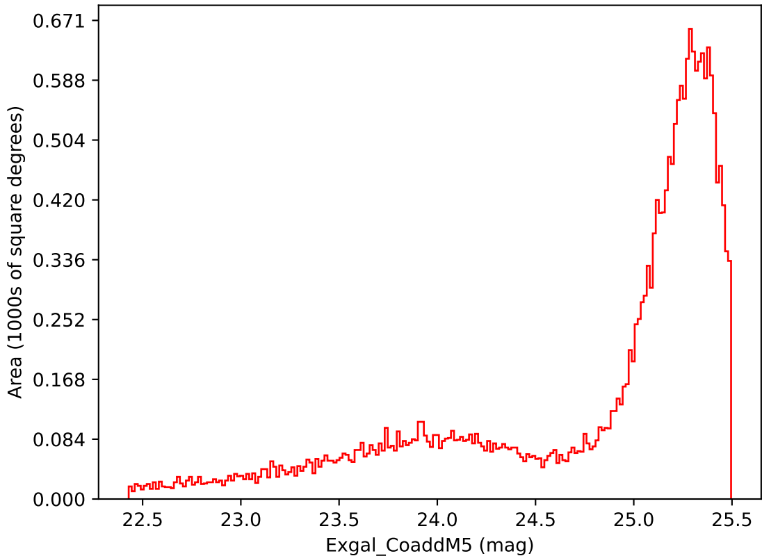
internal_u_expt30_nscale1.2v3.4_10yrs Yr 1 i band: Exgal_CoaddM5
