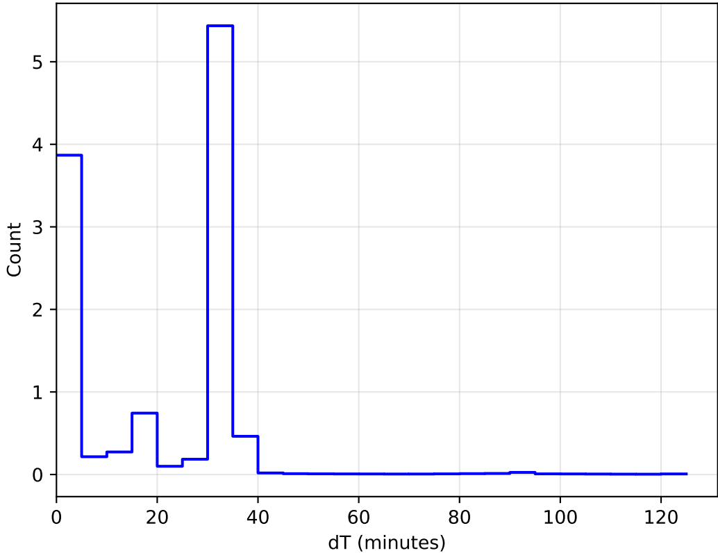
internal_u_expt30_nscale1.2v3.4_10yrs WFD: DeltaT Histogram
