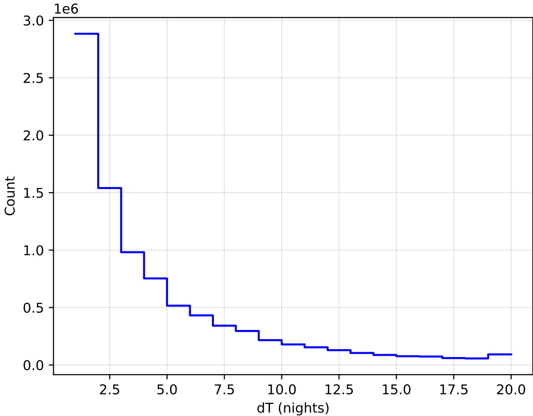
internal_u_expt30_nscale1.2v3.4_10yrs All sky all bands: DeltaNight Histogram
