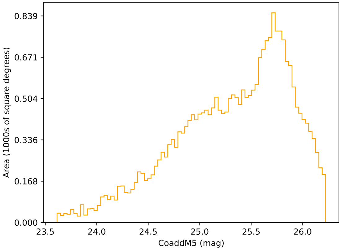
internal_u_expt30_nscale1.2v3.4_10yrs Yr 3-4 r band: CoaddM5
