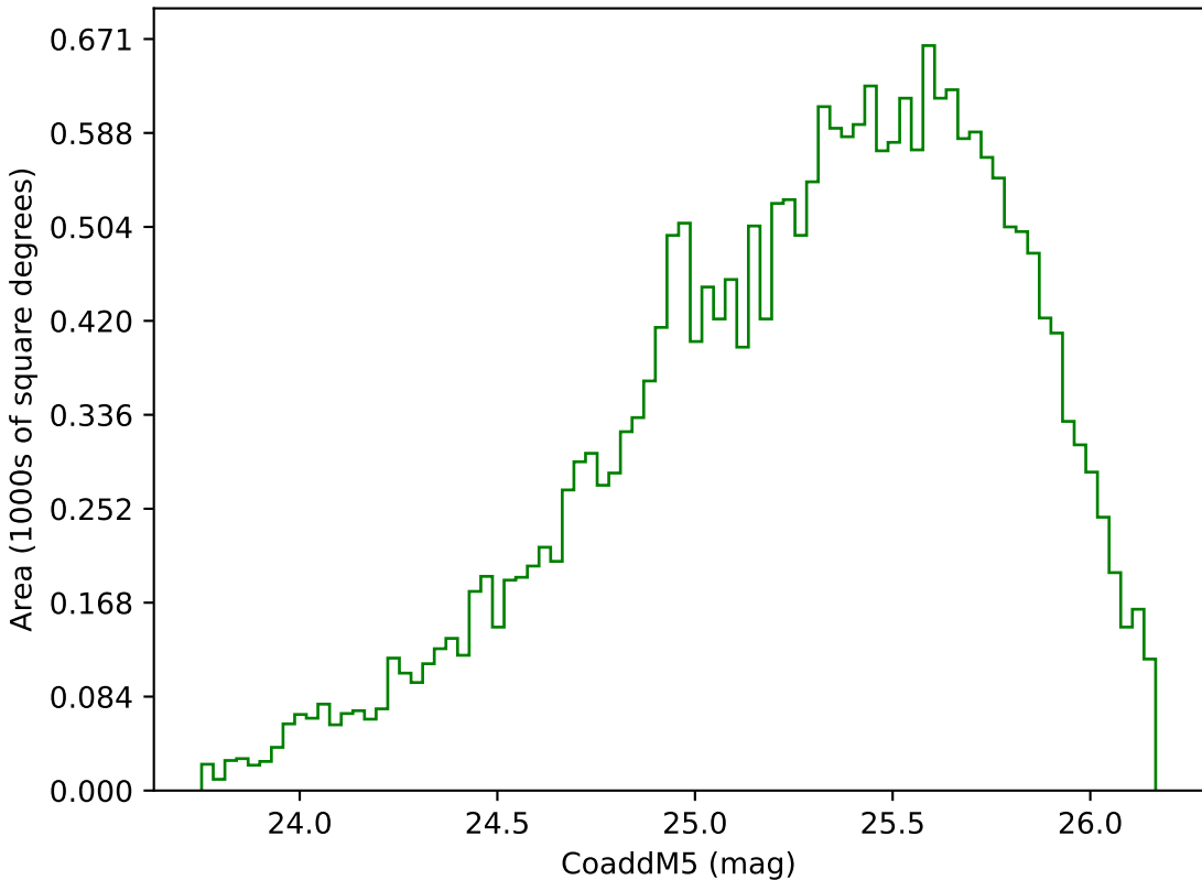
internal_u_expt30_nscale1.2v3.4_10yrs Yr 3-4 g band: CoaddM5
