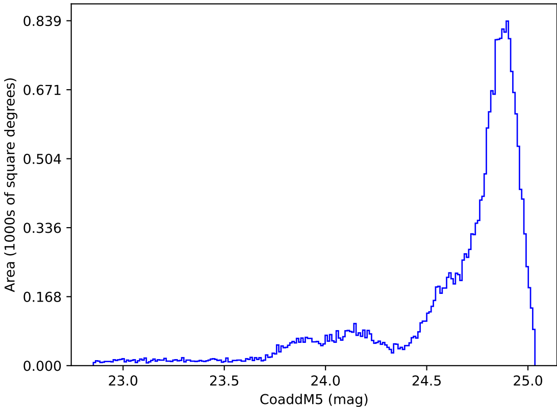
internal_u_expt30_nscale1.2v3.4_10yrs All sky y band: CoaddM5
