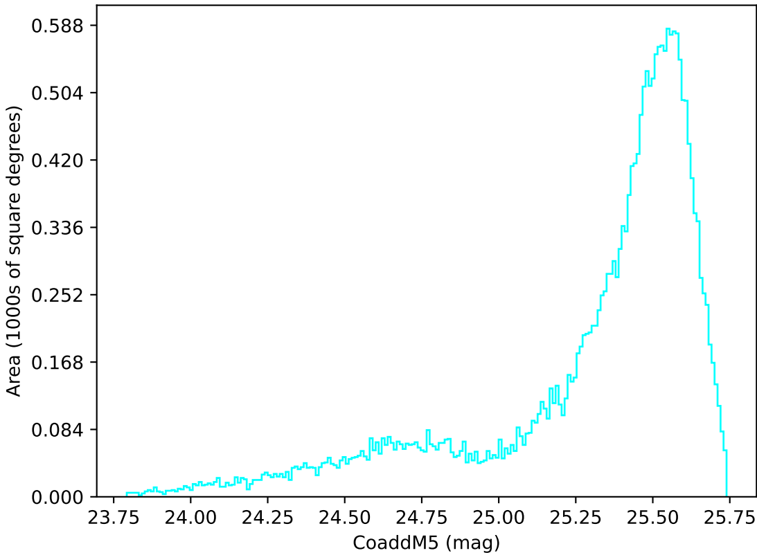
internal_u_expt30_nscale1.2v3.4_10yrs All sky u band: CoaddM5
