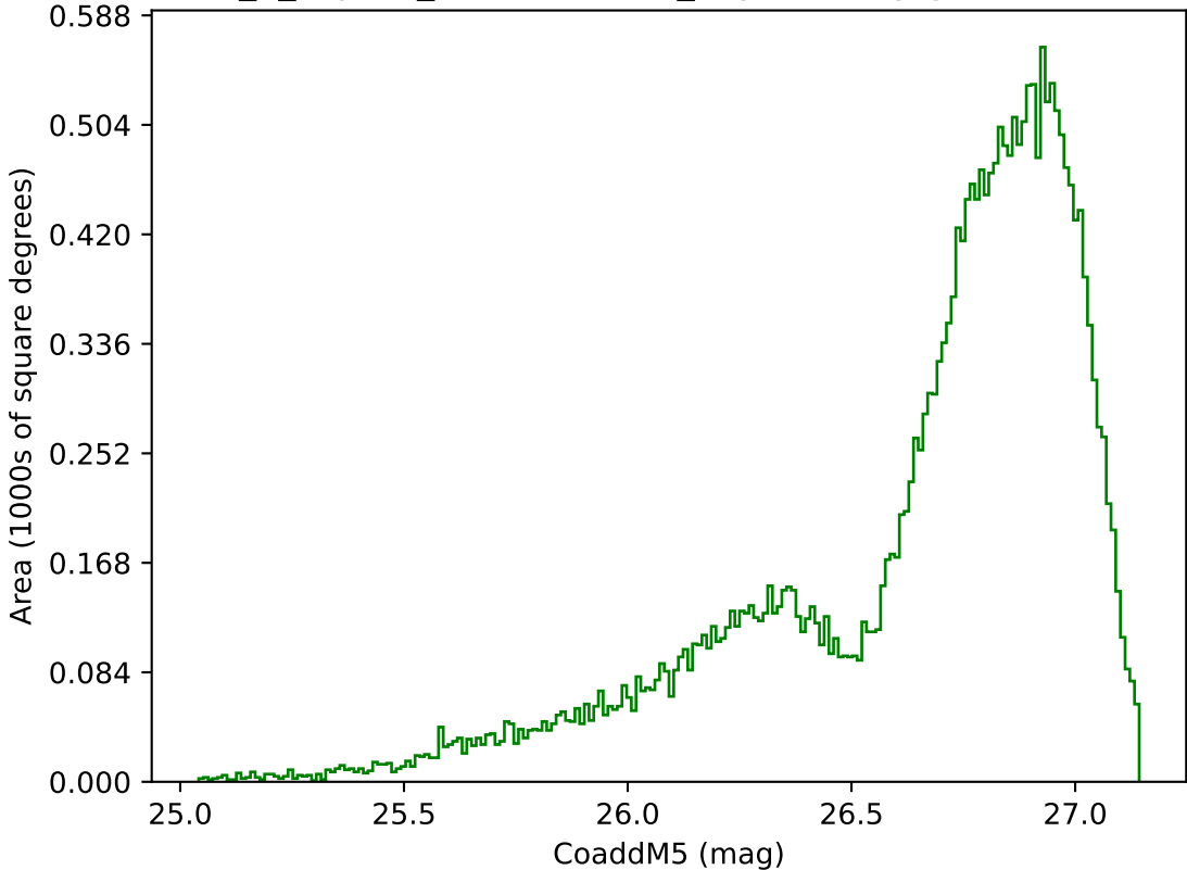
internal_u_expt30_nscale1.2v3.4_10yrs All sky g band: CoaddM5
