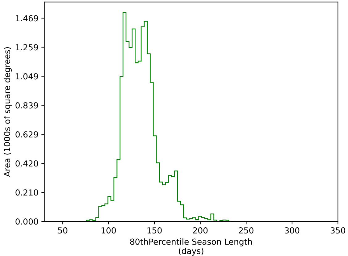
internal_u_expt30_nscale1.2v3.4_10yrs WFD g band: 80thPercentile Season Length
