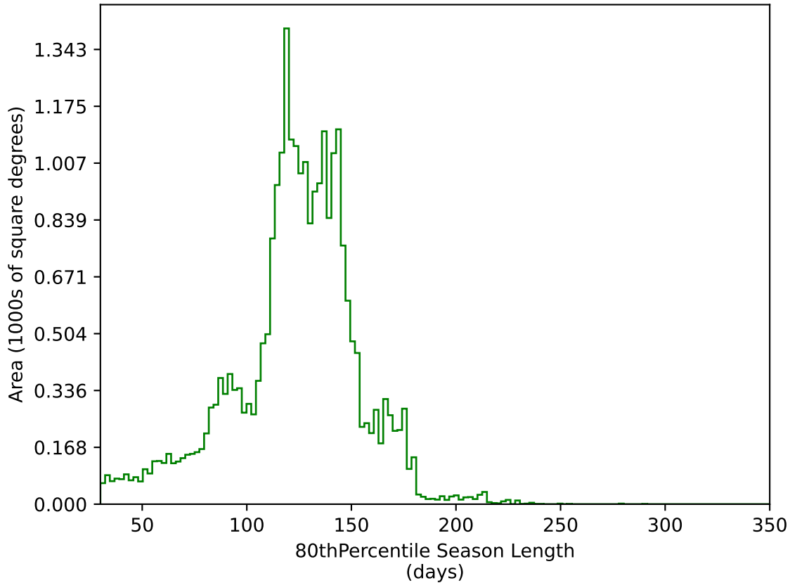
internal_u_expt30_nscale1.2v3.4_10yrs All sky g band: 80thPercentile Season Length
