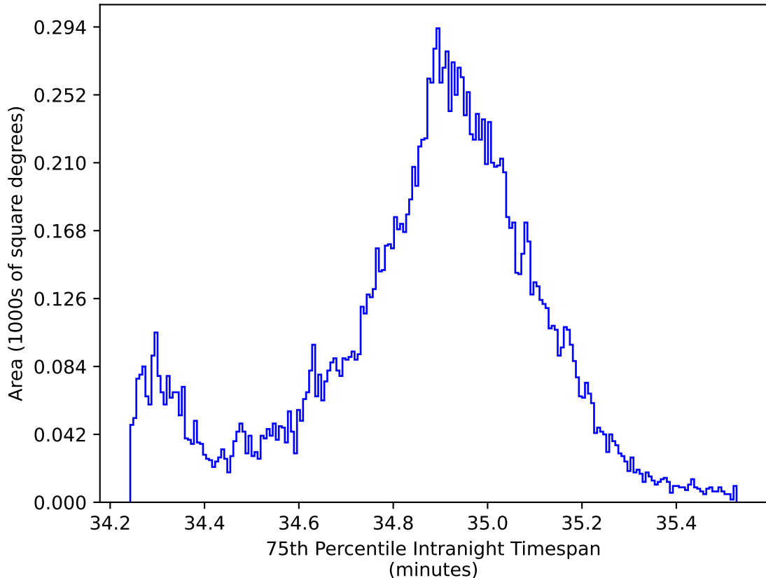
internal_u_expt30_nscale1.2v3.4_10yrs WFD all bands: 75th Percentile Intranight Timespan
