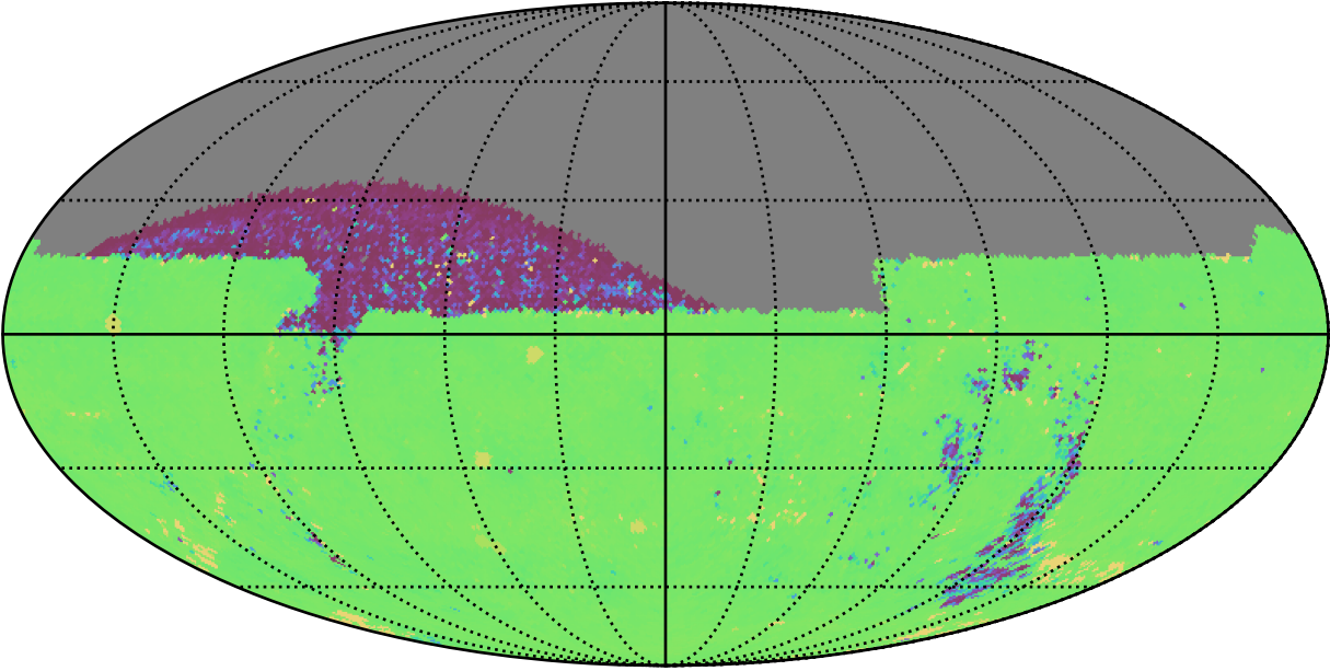
internal_u_expt30_nscale1.2v3.4_10yrs All sky ug bands: 75th Percentile Intranight Timespan
