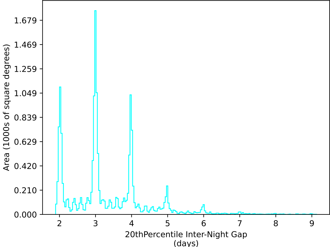
internal_u_expt30_nscale1.2v3.4_10yrs WFD u band: 20thPercentile Inter-Night Gap
