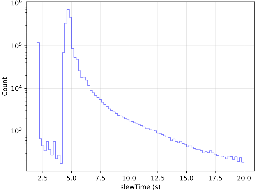
internal_u_expt30_nscale1.2v3.4_10yrs All visits: Zoom Slew Time Histogram
