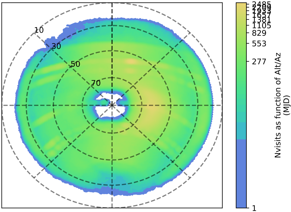
internal_u_expt30_nscale1.2v3.4_10yrs z: Nvisits as function of Alt/Az
