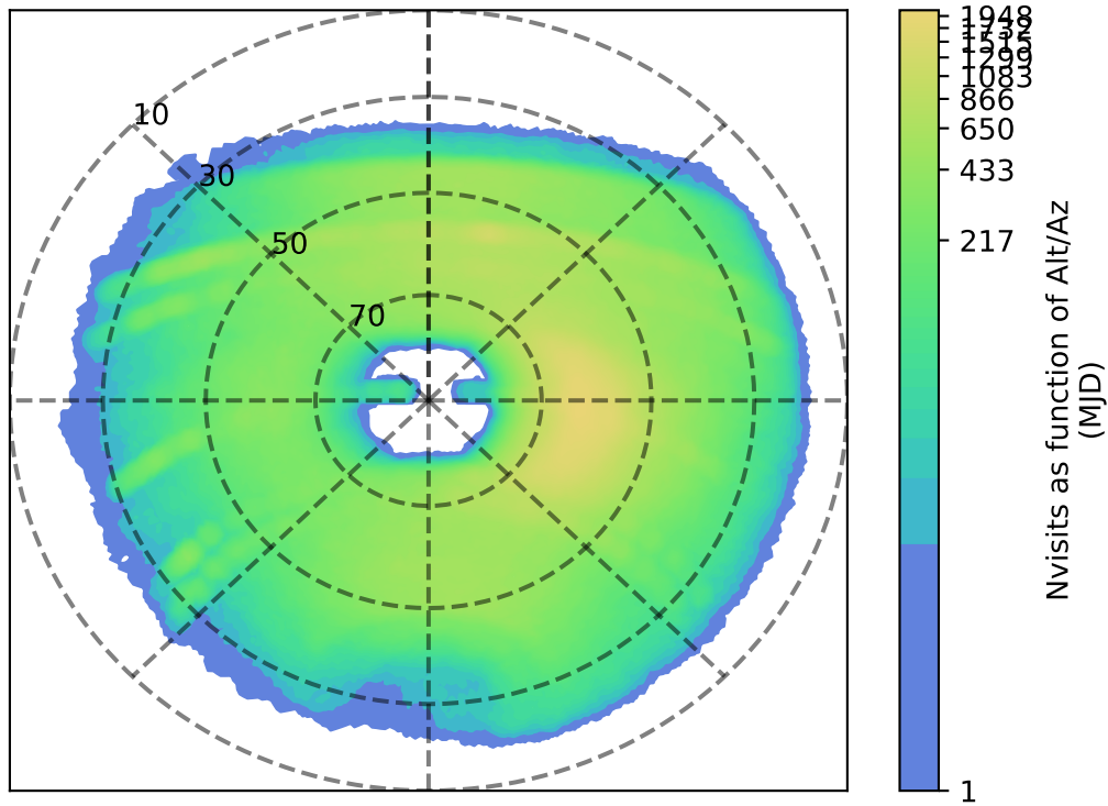
internal_u_expt30_nscale1.2v3.4_10yrs y: Nvisits as function of Alt/Az
